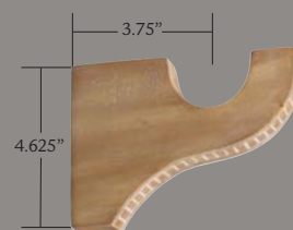
BRW178 small wall bracket
